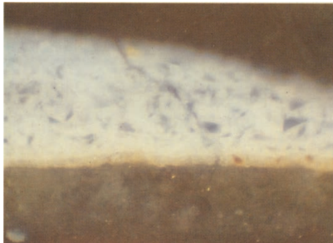
Fig. 9. Cross section ( 390\times ) from the whitish sky in no. A 5 (taken near the edge where it has been painted only once as opposed to the double layer elsewhere), showing: 1. the chalk and glue ground, 2. a thin layer of yellowish 'primuersel' (containing white lead and some brown pigment), 3. a layer of white lead, mixed with greyish particles (probably smalt)
